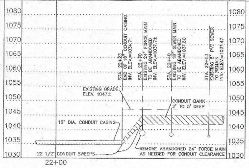
CONDUIT DETAILED PROFILE AT STA. 22+00 TO STA. 22+60 PROFILE SCALE: 1" = 10' HORIZONTAL 1" = 10' VERTICAL
